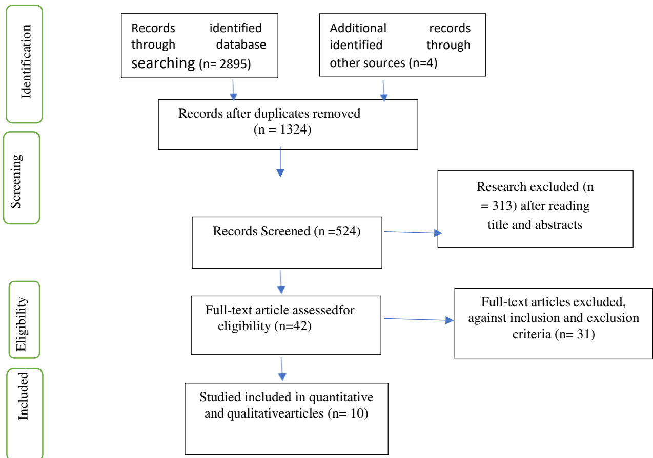
Figure 1: Data abstraction
